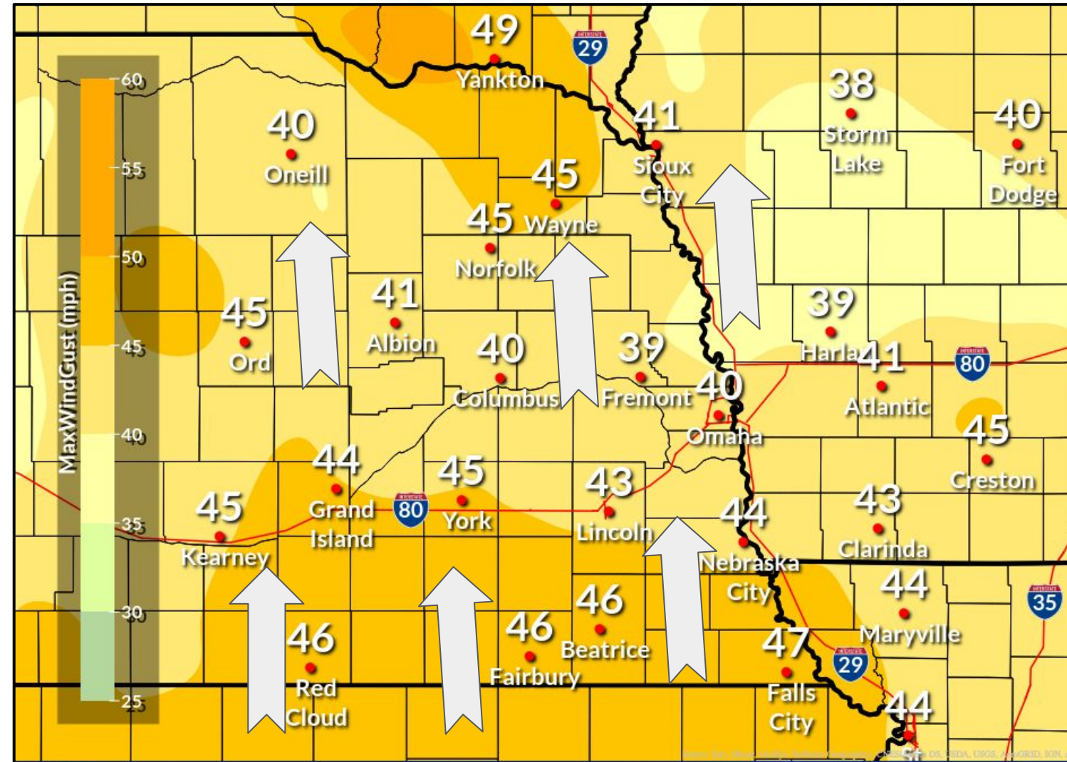
Strongest Wind Gusts Today
