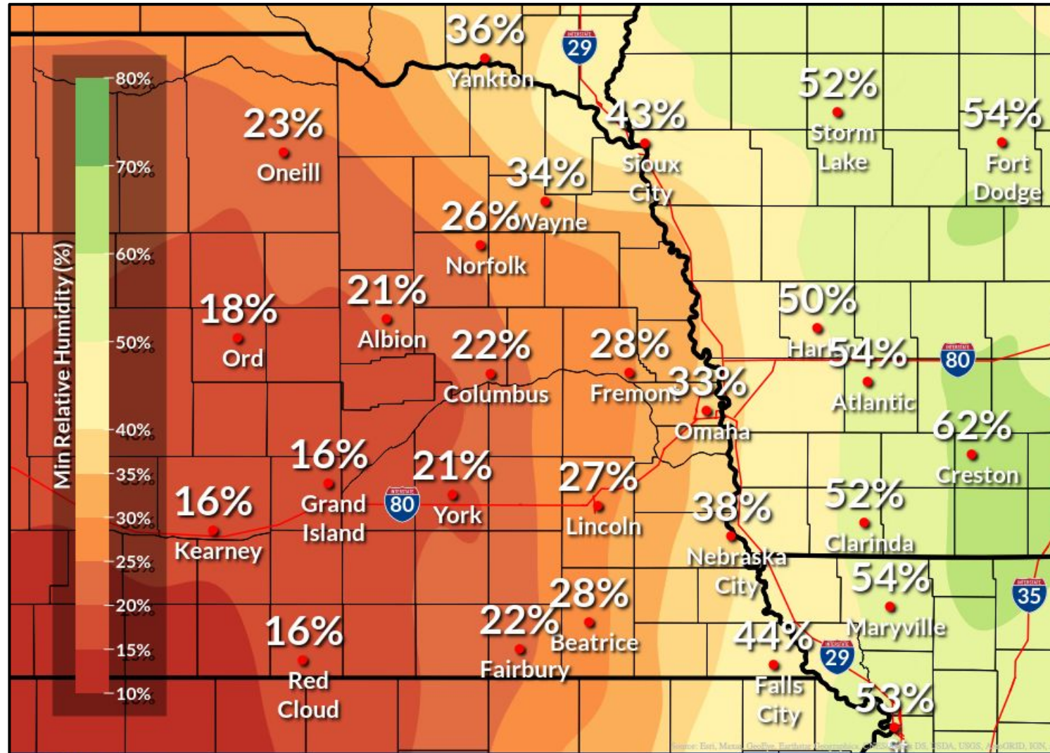
Minimum Relative Humidity Today
